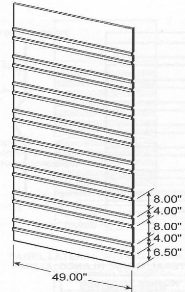
PANEL LATERAL SUPER SEAL, 16 CORR
