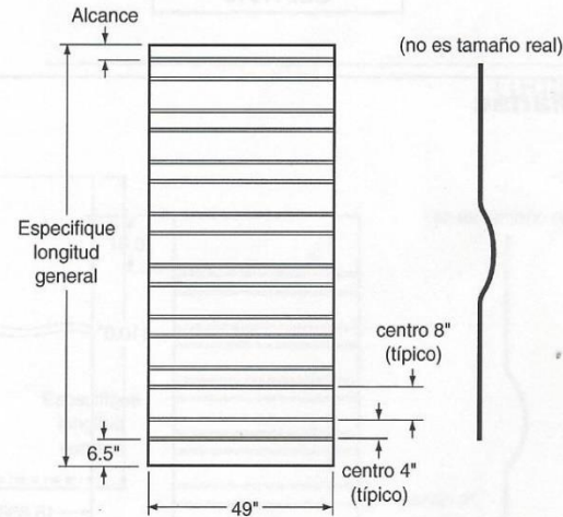
PANEL LATERAL, CORR, BLANCO, ALUM
