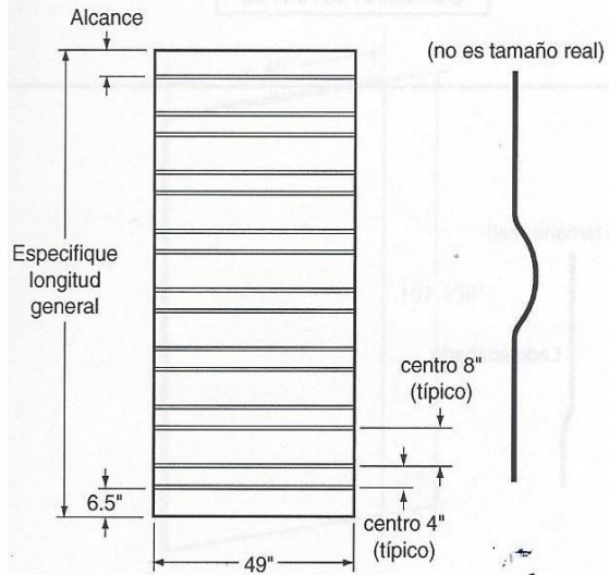
PANEL LATERAL, CORR, BLANCO, ALUM
