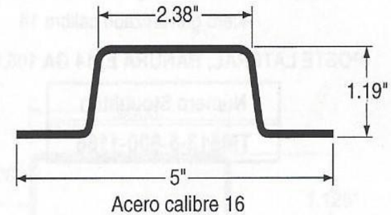
5" POSTE LATERAL, PERFORADO, 16 GA, 112"
